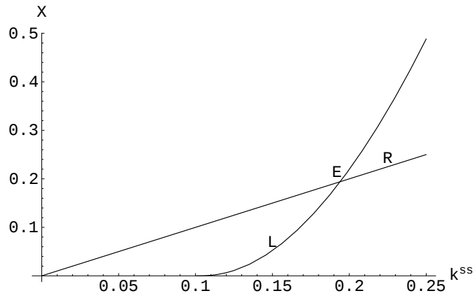
Figure 1: Steady-state Capital Stock
