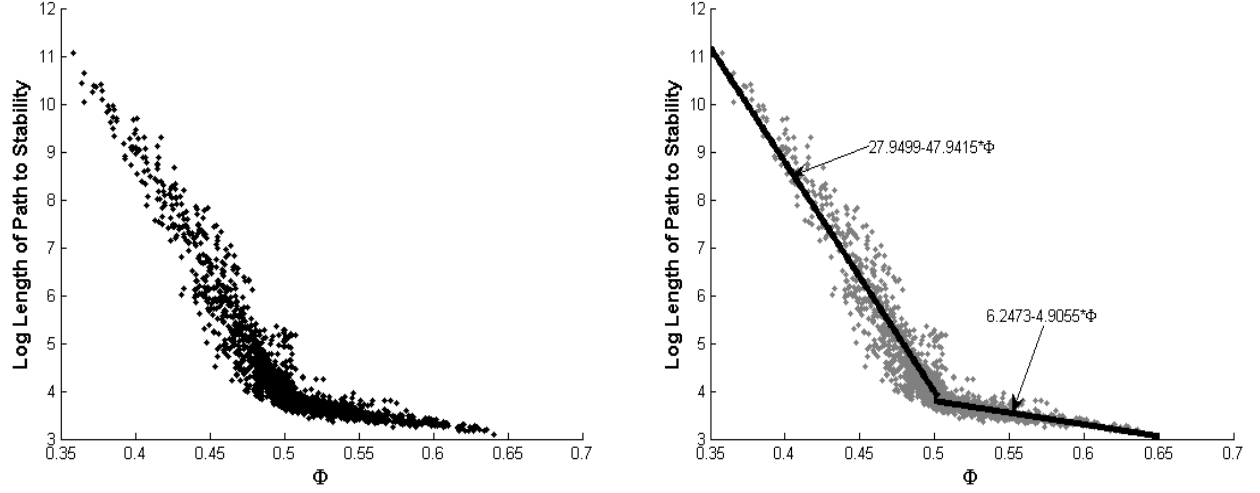
Figure 1: Simulation Results on Intercorelation
