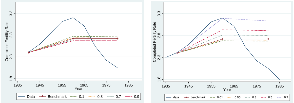
(a) Sensitivity Analysis Results: \sigma
