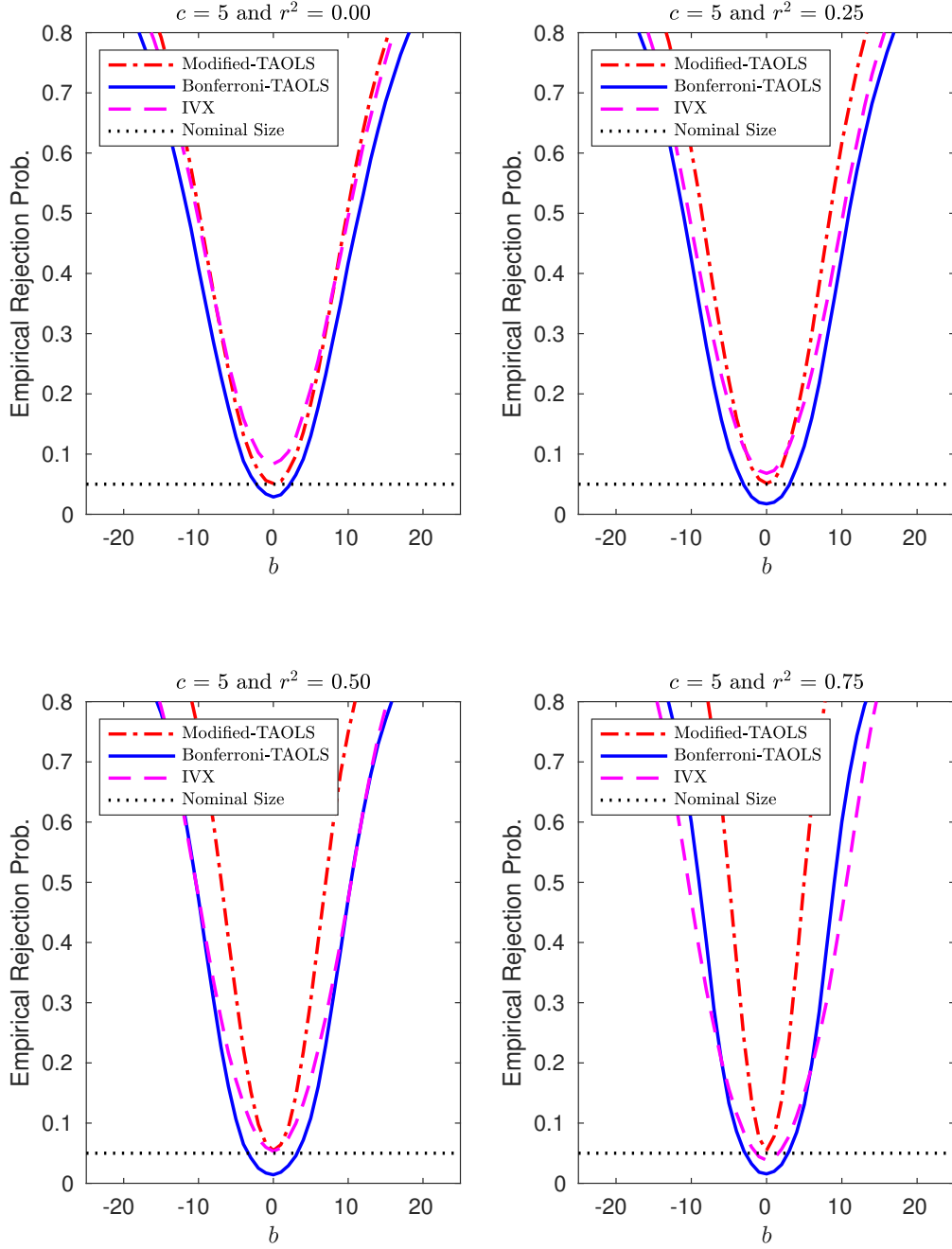
Figure 5: Finite sample power of 5% TA-OLS tests (Modified TAOLS and Feasible Bonferroni Modified TAOLS) and IVX test with K = 16 , c = 5 , and AR(1) error with \psi = 0.25 .
