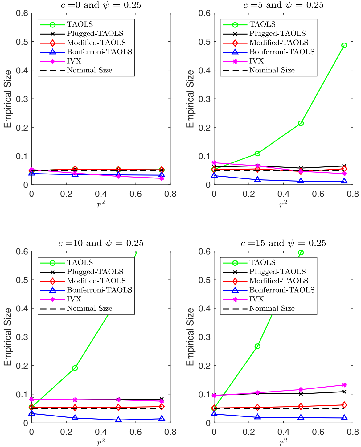
Figure 3: Empirical size of 5% fixed-smoothing tests (TA-OLS, Infeasible Plugged-in TA-OLS, Infeasible Modified TAOLS, and Feasible Bonferroni Modified TA-OLS, IVX) with K = 24 and AR(1) error with \psi = 0.25 , and single regressor.
