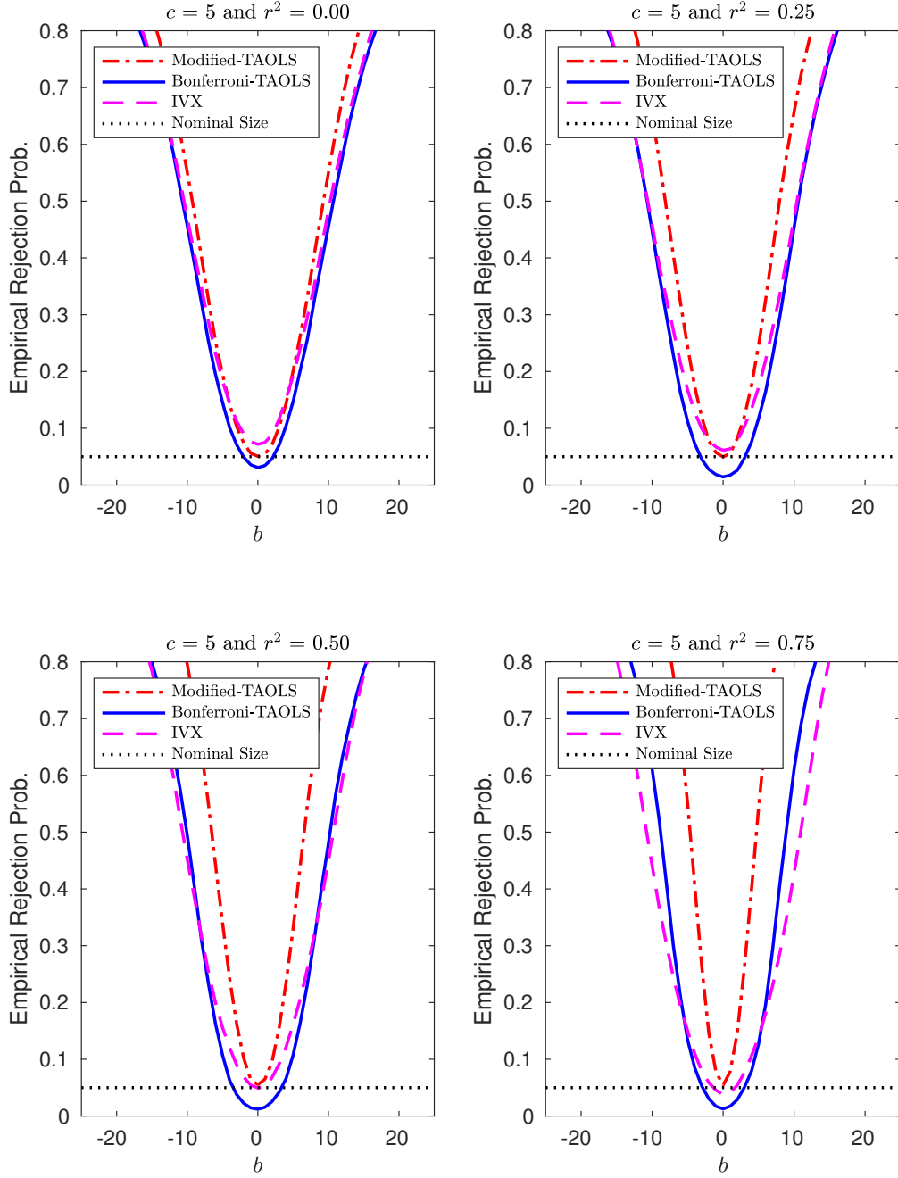
Figure 4: Finite sample power of 5% TA-OLS tests (Modified TAOLS and Feasible Bonferroni Modified TAOLS) and IVX test with K = 24 , c = 5 , and AR(1) error with \psi = 0.25 .
