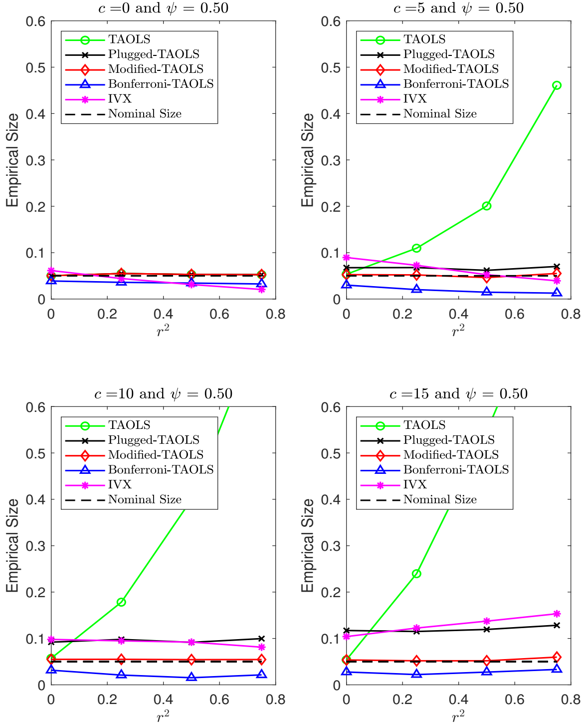
Figure 2: Empirical size of 5% fixed-smoothing tests (TA-OLS, Infeasible Plugged-in TA-OLS, Infeasible Modified TAOLS, and Feasible Bonferroni Modified TA-OLS, IVX) with K = 16 and AR(1) error with \psi = 0.50 , and single regressor.
