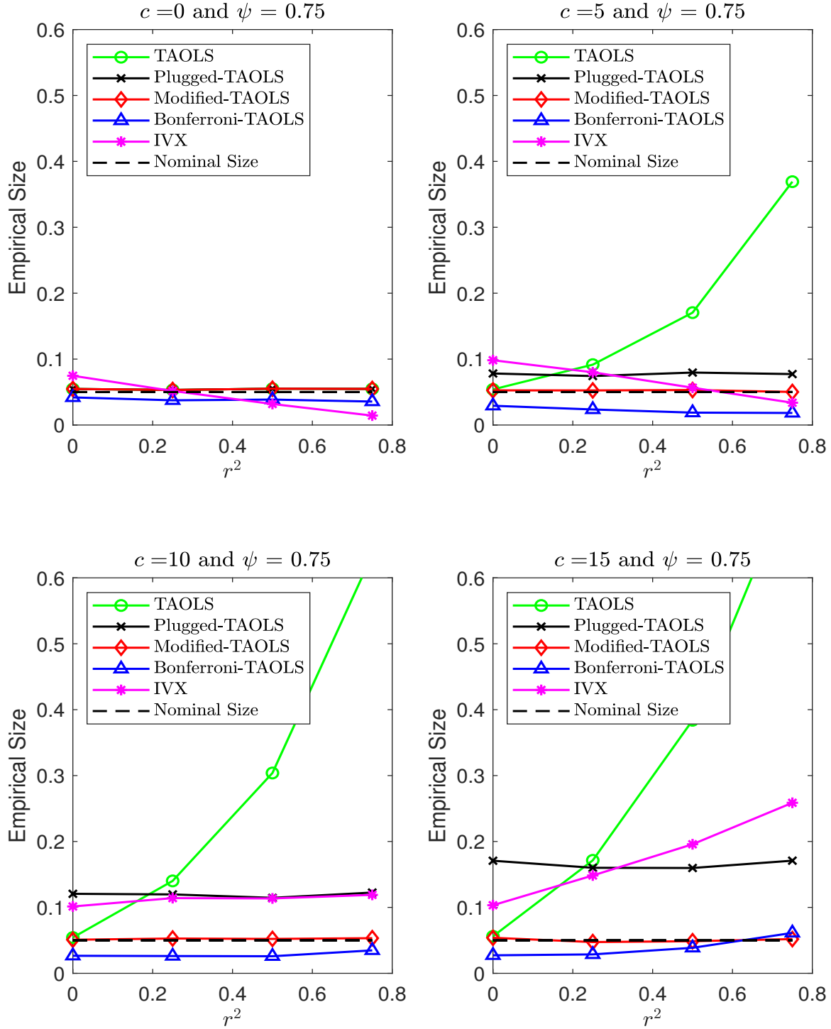
Figure 1: Empirical size of 5% fixed-smoothing tests (TA-OLS, Infeasible Plugged-in TA-OLS, Infeasible Modified TAOLS, and Feasible Bonferroni Modified TA-OLS, IVX) with K = 8 and AR(1) error with \psi = 0.75 , and single regressor.
